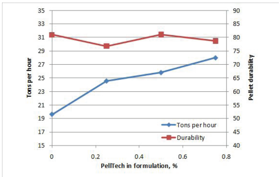
Figure 3 – Production increase with varied levels of PellTech at 70% load.
